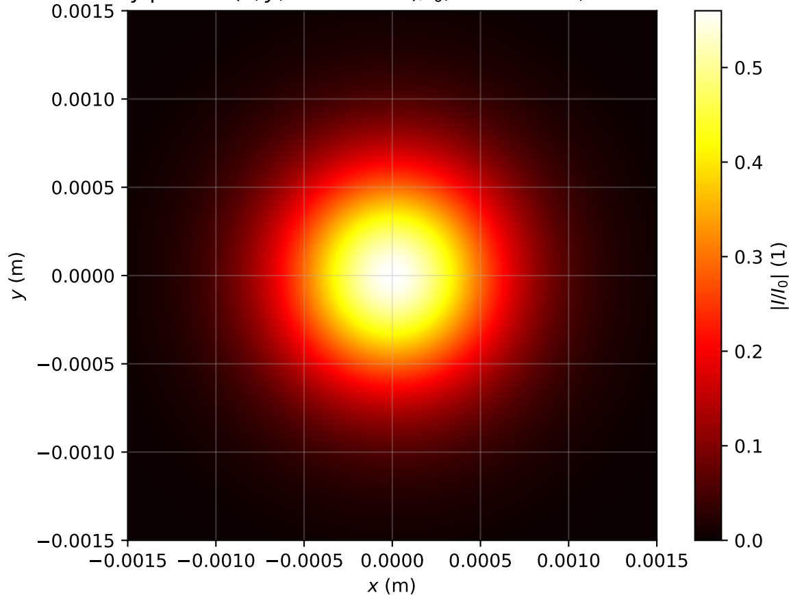
Intensity profile I(x, y, z = 3.025m)/I_0 , Pin=0.5Pcr, artificial time
